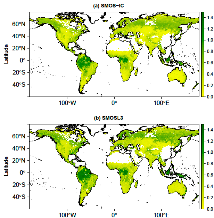
Figure 6. Temporal mean of \tau during 2010–2015: (a) SMOS-IC; and (b) SMOSL3.
