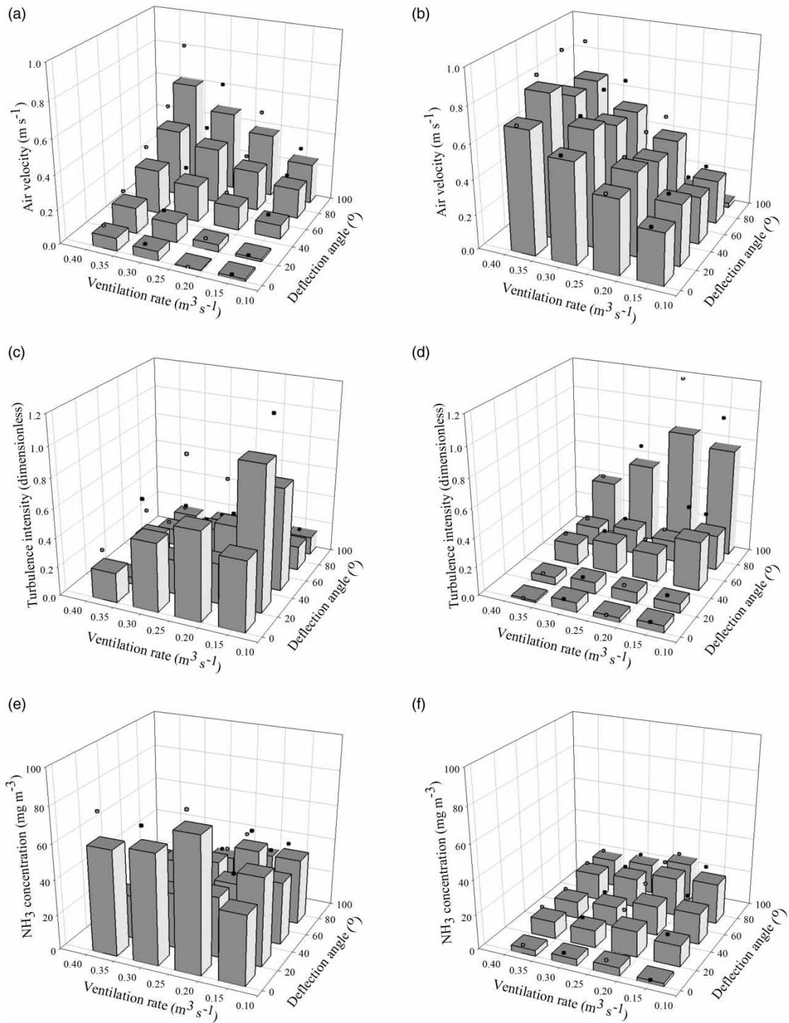
Figure 4. Air velocity ( u , \text{m s}^{-1} ; a and b), TI (dimensionless; c and d) and \text{NH}_3 concentration ( [\text{NH}_3] , \text{mg m}^{-3} ; e and f) plotted against VR ( \text{m}^3 \text{s}^{-1} ) and DA ( ^\circ ). Charts to the left refer to variables monitored between slats and the charts to the right are for variables measured at 0.25 m above the slats. Dots placed above each bar represent the upper limit of the 95% confidence interval.
