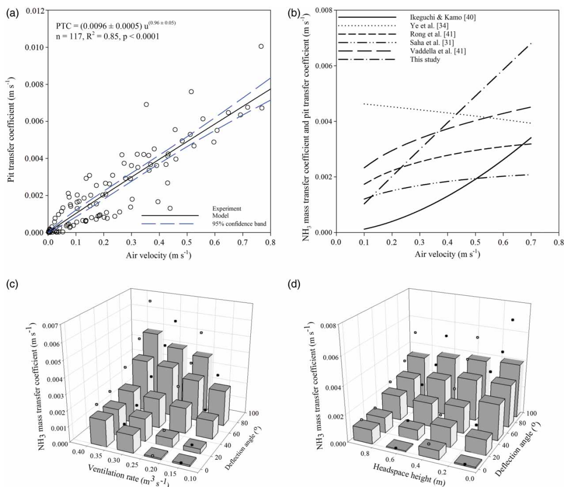
Figure 6. Regression curve for PTC of NH_3 ( m s^{-1} ) (a); PTC curve from this study plotted together with NH_3 mass transfer coefficients ( k_{NH_3} , m s^{-1} ) from other studies (b). Bar charts of the effects of VR ( m ) versus DA ( ^\circ ) on PTC , and (c) and of the effects of HH ( m ) versus DA (d) on PTC , m s^{-1} , monitored in the test section of the wind tunnel. Dots placed above each bar represent the upper limit of the 95% confidence interval.
