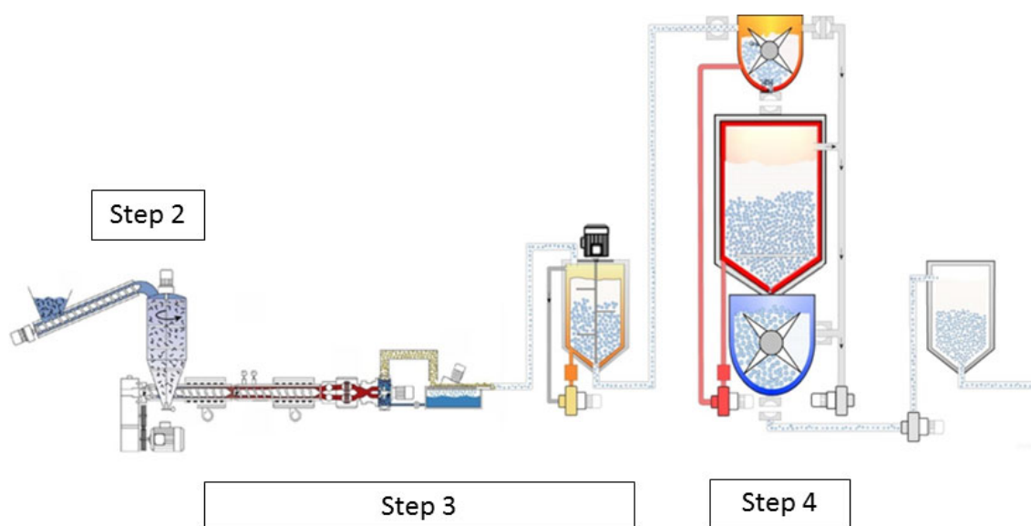
Figure 1: General scheme of the Starlinger IV+ ® technology
