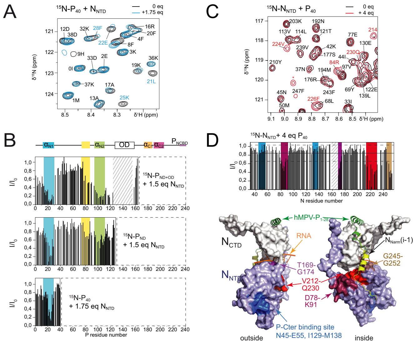
FIGURE 5. Interaction between hRSV N_{NTD} and the N terminus of P. A , selected region of the ^1\text{H} - ^{15}\text{N} HSQC spectrum of ^{15}\text{N} - P_{40} in the presence or absence of N_{NTD} . B , intensity ratios ( I/I_0 ) measured from ^1\text{H} - ^{15}\text{N} HSQC spectra of ^{15}\text{N} -labeled N-terminal fragments of P in the presence of N_{NTD} . The hatched area indicates missing signals in the free forms. The background is colored according to transient secondary structures as indicated above. C , selected region of the ^1\text{H} - ^{15}\text{N} HSQC spectrum of ^{15}\text{N} - N_{NTD} in the presence or absence of P_{40} . D , intensity ratios for ^{15}\text{N} - N_{NTD} in the presence of P_{40} measured from C . Full and broken horizontal lines indicate the mean \pm S.D., respectively. Regions with significant line broadening ( I/I_0 < \text{mean} - 1 \text{ S.D.} ) are highlighted by red to brown backgrounds and the P C terminus binding region by blue color (39). The hatched area corresponds to unassigned N_{NTD} residues Ile 160 -Val 167 . The same color code is used to map these regions on the three-dimensional structure of an N protomer of N-RNA rings (PDB 2WJ8). The two views in surface representation are rotated by 180° and show the outside and inside of the N-RNA ring. The N-terminal arm (Ala 2 -Gly 30 ) of the preceding N protomer in the ring (i-1) is in yellow schematic. The N-terminal P_{1-28} peptide of the hMPV N^0 -P complex (PDB 5FVD) (40) in green schematic was superimposed onto hRSV N.
