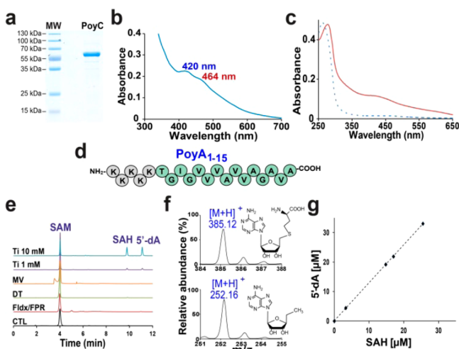
Figure 2. (a) Gel electrophoresis analysis of PoyC (SDS PAGE 12%). (b) UV-vis spectrum of as-isolated PoyC. (c) UV-vis spectra of PoyC before (dashed line) and after (solid line) iron-sulfur reconstitution. (d) Sequence of the PoyA 1-15 peptide used as the substrate. (e) HPLC analysis of PoyC reactions after incubation under anaerobic conditions with SAM (2 mM), DTT (6 mM), and PoyA 1-15 (1 mM) in the presence of various reductants, including sodium dithionite (DT), flavodoxin/flavodoxin reductase/NADPH (Fldx/FPR), methyl viologen/NADPH (MV), titanium citrate (Ti), or in the absence of reductant (CTL) (UV detection at 257 nm). See the Supporting Information (SI) for the experimental conditions. (f) MS analyses of SAH (upper trace) and 5'-dA (lower trace) produced by PoyC. (g) Correlation between SAH and 5'-dA produced by PoyC. Analyses were performed between 0 and 20 min as described in the SI.
