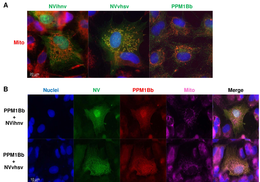
Figure 6. PPM1Bb is co-localized with both NV proteins in close proximity to mitochondria. EPC cells were transfected with 1.5 µg of the indicated plasmids alone (A) and in combination (B) for 24 h. Cell mitochondria were then stained with a red MitoTracker. After fixation and permeabilization, PPM1Bb and NV proteins were detected with anti-HA and anti-Flag mAbs, respectively. The nuclei were stained with DAPI (blue).
