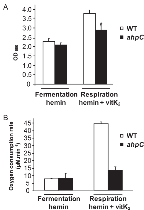
FIGURE 4. GBS respiration metabolism is attenuated in an ahpC mutant. A , growth of WT and ahpC GBS in respiration-permissive conditions. WT and ahpC GBS strains were grown for 5–6 h in aerated or respiration-permissive (1 \mu\text{M} hemin and 10 \mu\text{M} vitamin K 2 ( vitK 2 )) or nonpermissive (1 \mu\text{M} hemin only) conditions in M17 supplemented with 1% glucose. The growth increase under respiration conditions was less pronounced for the ahpC GBS mutant. Results represent the means \pm S.D. from at least 10 independent experiments. Asterisk denotes statistically significant reduction of respiration in the ahpC mutant compared with the WT as determined by Student's t test ( p < 0.05 ). B , comparative oxygen consumption rates in WT and ahpC mutants grown as in Fig. 5 A . Oxygen consumption was measured on whole cells grown under aerobic fermentation and respiration conditions with a Clark-type electrode as described under "Experimental Procedures." Oxygen consumption, which is characteristic of respiration metabolism when oxygen is the terminal electron acceptor, was markedly reduced in the ahpC mutant, showing that respiration rate is decreased. Data are normalized to A_{600} = 1 for both cultures and are means \pm S.D. from three experiments.
