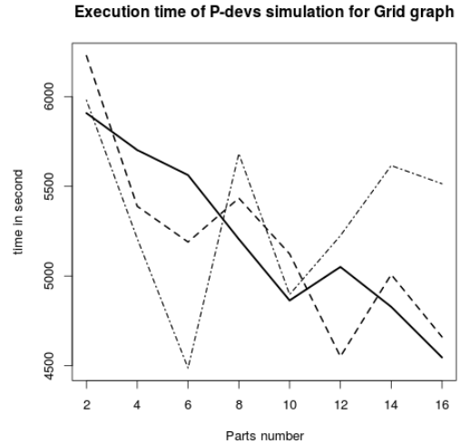
Figure 7. Evolution of parallel simulation time against part number for a grid graph
