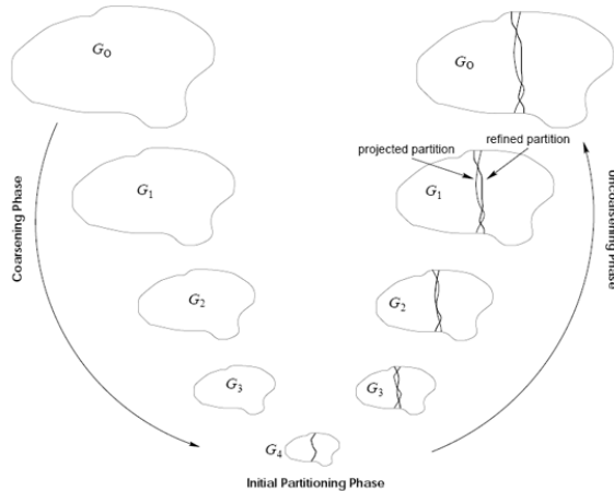
Figure 2. Multilevel Graph Bisection
