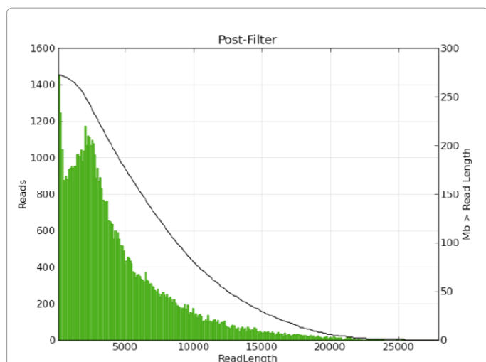
Distribution of subreads obtained after filtration (Assembly workflow on Figure 5) shows a pic shorter reads around 2500 bp. Shorter reads are used to correct error of the longer subreads (>11 kbp).
