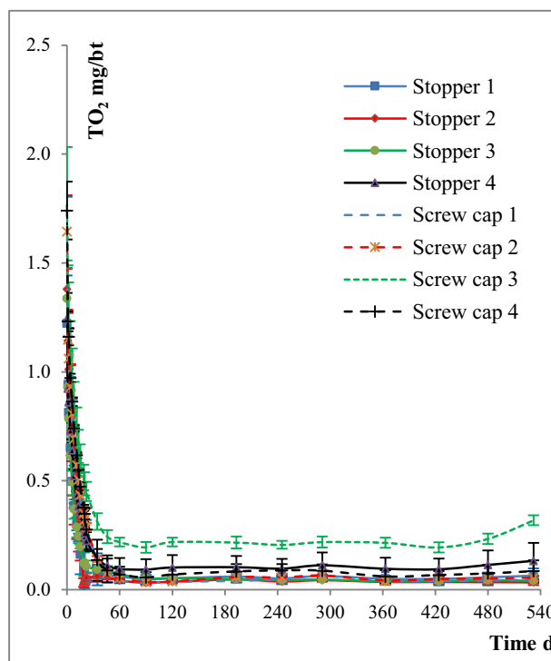
Figure 1. TO 2 = f(t) for each procedure. TO 2 mg/bt: Total oxygen in mg/bottle. Averages and standard deviations are based on 3 bottles per procedure.
