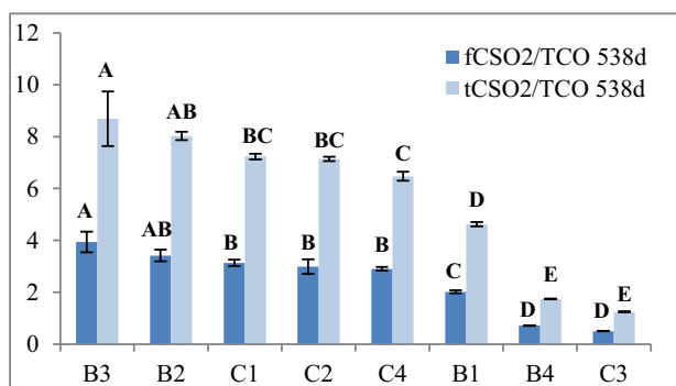
Figure 3. Ratios of free/total Consumed SO 2 / TCO at 538 days. Stoppers B1 to B4; screw caps C1 to C4. f(t)CSO 2 /TCO: free (total) Consumed SO 2 / Total Consumed Oxygen. fCSO 2 , tCSO 2 and TCO expressed in mg/L. Ratios ranked in descending order of fCSO 2 /TCO 538 d. Different labels (A, B, C, D, E) indicate means that significantly differ at p<0.0001. Averages and standard deviations are based on 3 bottles per procedure.
