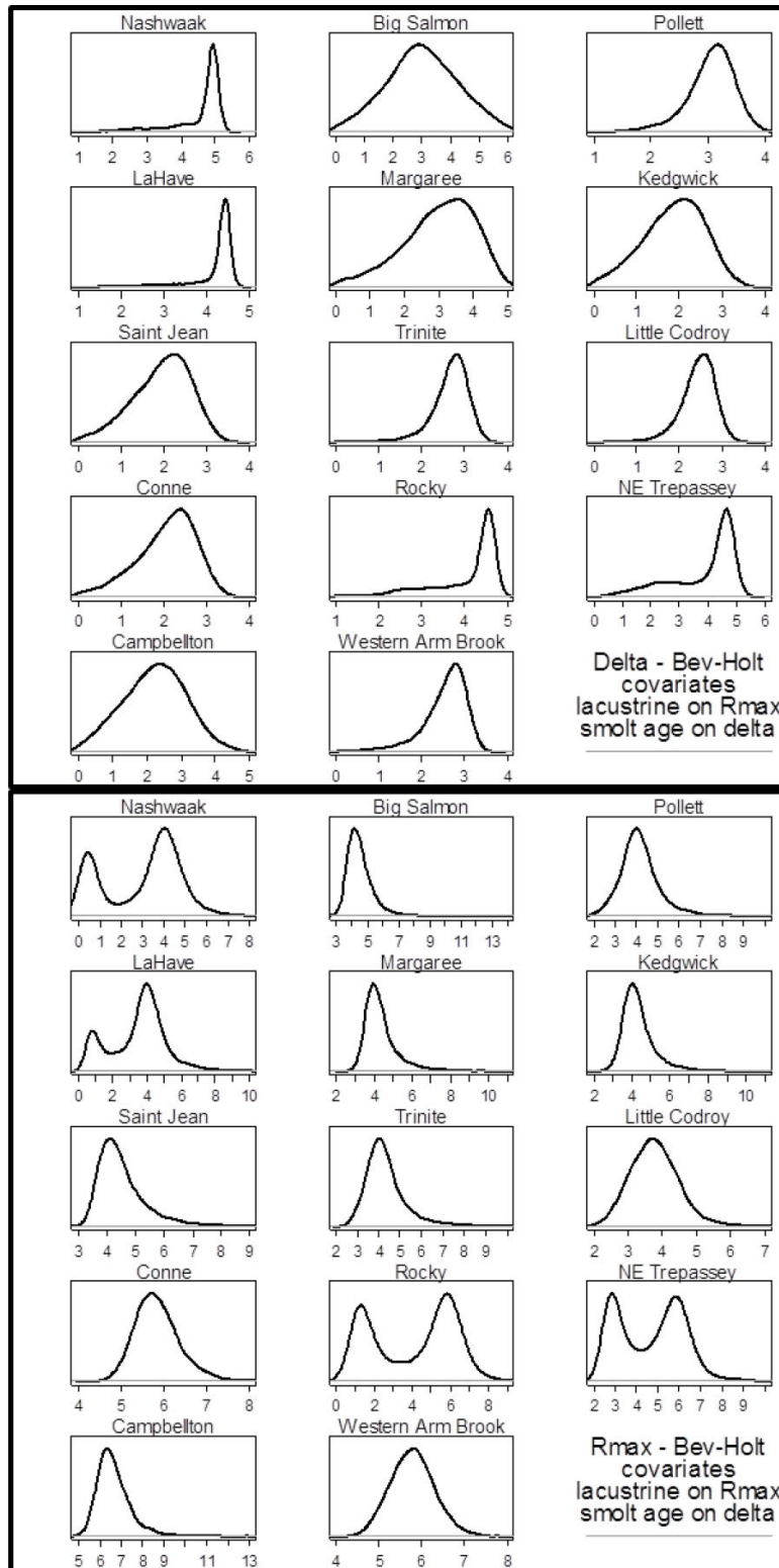
Figure 27. Posterior distributions of \delta (upper panel) and R_{max} (lower panel) from the Beverton-Holt hierarchical model on \sigma , with lacustrine presence as covariate on R_{max} and mean age of smolts as covariate on \delta .
