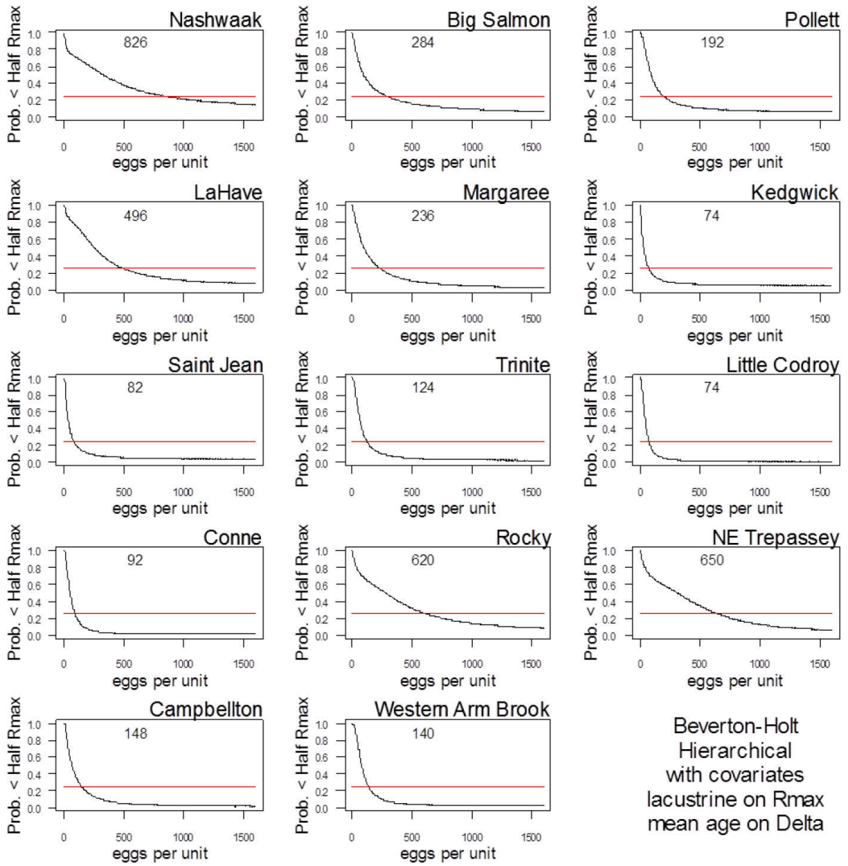
Figure 33. Eggs depositions versus probability that smolts produced will be < Half Rmax, taking into account the uncertainty of the stock and recruitment relationships and the estimated process error (sigma). Values on each panel are the eggs corresponding to a probability of ~ 0.25 of recruitment being below Half Rmax ( S_{LRP} ).
