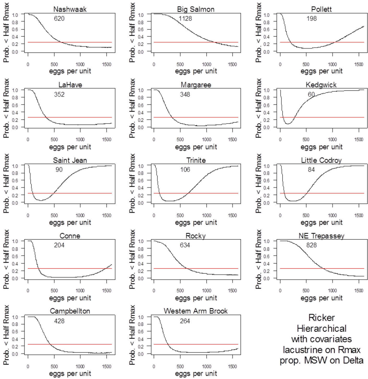
Figure 43. Eggs depositions versus probability that smolts produced will be < \text{Half } R_{\text{max}} , taking into account the uncertainty of the Ricker stock and recruitment relationships and the estimated process error ( \sigma ). Values on each panel are the eggs corresponding to a probability of \sim 0.25 of recruitment being below \text{Half } R_{\text{max}} ( S_{LRP} ).
