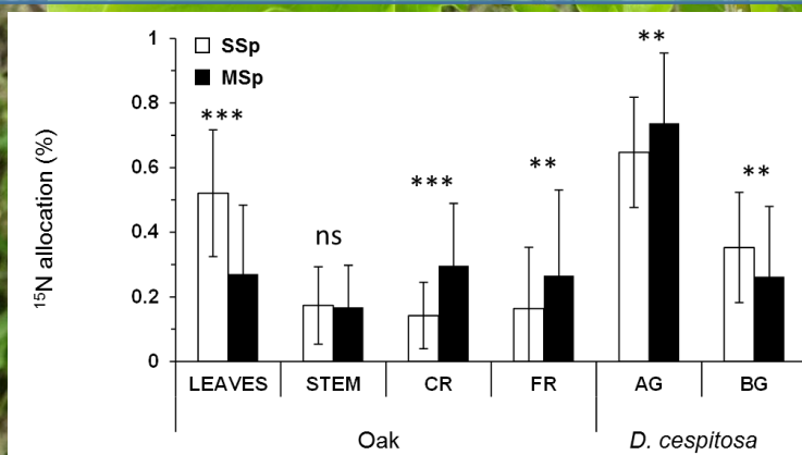
Fig 2: Relative allocation of 15 N among leaves, stems, coarse (CR) and fine roots (FR) in oak seedlings and D. cespitosa (above ground biomass (AG) and below ground biomass (BG)) when sole- (SSp) or mixed-grown (MSp)
