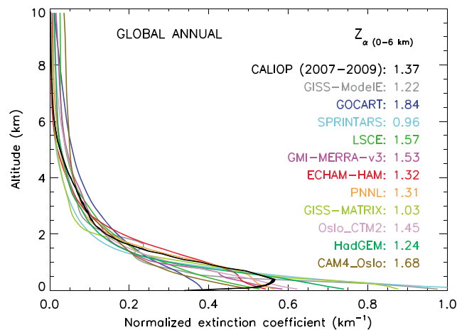
Figure 4. Models (2006) and CALIOP (2007–2009) global mean annual “normalized” extinction coefficient ( \text{km}^{-1} ) profiles (at 550 and 532 nm, respectively). The 2007 to 2009 range is shown for CALIOP (black). The simulated and observed Z_{\alpha 0-6 \text{ km}} mean extinction heights (km) are also reported. See Tables 1a, 1b, 1c for the definition of the models.
