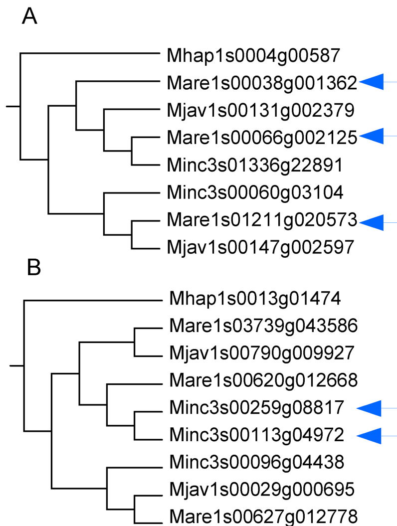
Fig 6. Allele-like versus homeologous relationship between genes in more than two copies. (A) An example of homeoeologous relationship where each M. arenaria gene copy (arrows) clusters with the copy of another species. (B) An example of allele-like relationship where two of the three M. incognita gene copies (arrows) are more similar to one another than they are to a copy from another species.
