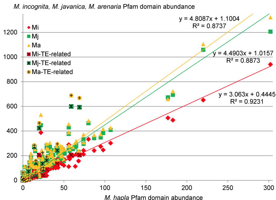
Fig 10. Pfam domain abundance in asexual Meloidogyne as a function of the abundance in M. hapla . The x-axis represents abundance of Pfam domains in M. hapla and the y-axis represents abundance of the same domains in M. incognita (red diamonds) M. javanica (green squares) and M. arenaria (yellow triangles). Linear regressions of M. incognita , M. javanica and M. arenaria Pfam domain abundances as a function of the abundance in M. hapla are plotted alongside their respective equations and correlation coefficients. Pfam domains associated to transposable elements (TE) are represented as crossed red, green and yellow squares in M. incognita , M. javanica and M. arenaria , respectively.
