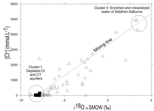
Figure 13. Chloride concentration versus \delta^{18}\text{O} in the Continental Intercalaire (filled squares), Complex Terminal (open circles) and phreatic (open triangles) aquifers from Ouargla.
