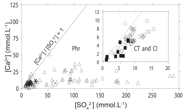
Figure 12. Calcium versus \text{SO}_4^{2-} diagram in the Continental Intercalaire (filled squares), Complex Terminal (open circles) and phreatic (open triangles) aquifers. Seawater composition (star) is [\text{Ca}^{2+}] = 10.2 \text{ mmol L}^{-1} and [\text{SO}_4^{2-}] = 28.2 \text{ mmol L}^{-1} (Stumm and Morgan, 1999, p. 899).
