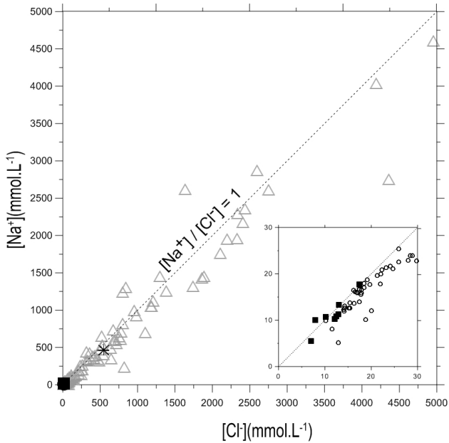
Figure 10. Correlation between \text{Na}^+ and \text{Cl}^- concentrations in the Continental Intercalaire (filled squares), Complex Terminal (open circles) and phreatic (open triangles) aquifers. Seawater composition (star) is [\text{Na}^+] = 459.3 \text{ mmol L}^{-1} and [\text{Cl}^-] = 535.3 \text{ mmol L}^{-1} (Stumm and Morgan, 1999, p. 899).
