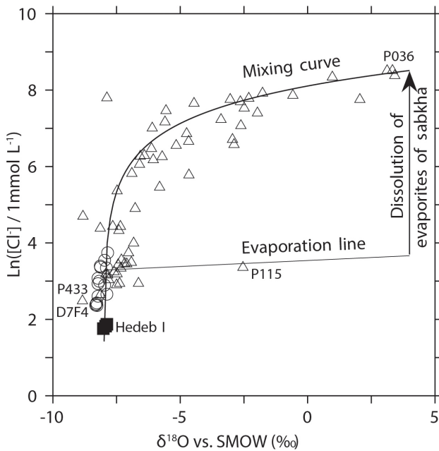
Figure 14. Log [Cl^-] concentration versus \delta^{18}O in Continental Intercalaire (filled squares), Complexe Terminal (open circles) and phreatic (open triangles) aquifers from Ouargla.
