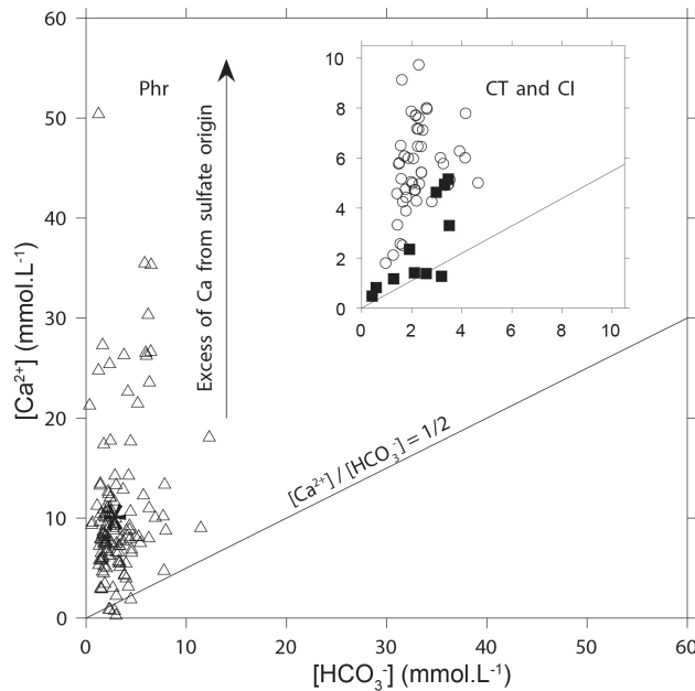
Figure 11. Calcium versus \text{HCO}_3^- diagram in the Continental Intercalaire (filled squares), Complex Terminal (open circles) and phreatic (open triangles) aquifers. Seawater composition (star) is [\text{Ca}^{2+}] = 10.2 \text{ mmol L}^{-1} and [\text{HCO}_3^-] = 2.38 \text{ mmol L}^{-1} (Stumm and Morgan, 1999, p. 899).
