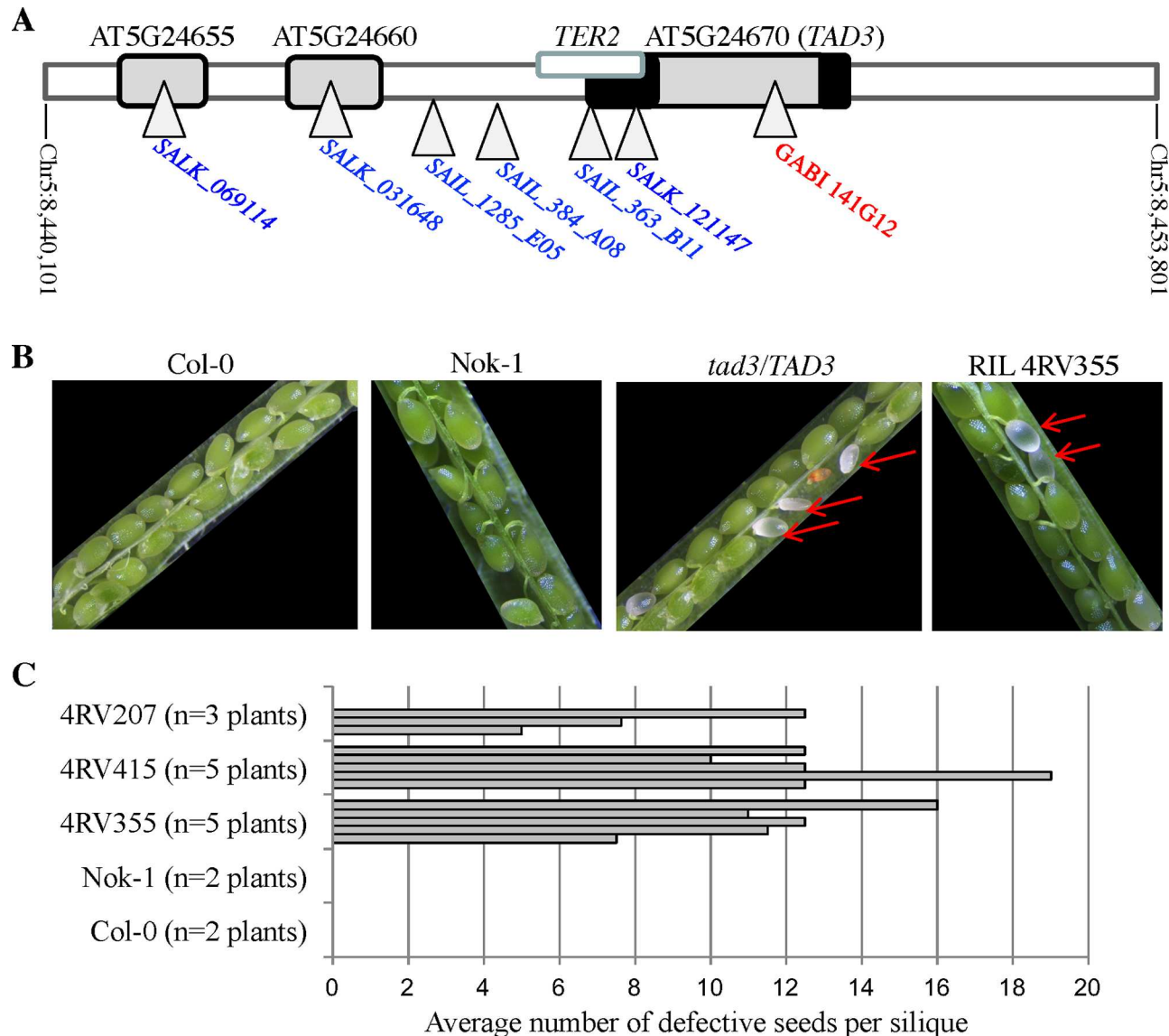
Fig 1. TAD3 is the candidate gene for the incompatibility between Nok-1/Est-1 and Col-0 . (A) The mapping interval localized on chromosome 5 in Col-0 contains four predicted genes. TER2 encodes a non-coding RNA associated with the telomerase [24]. AT5G24655 and AT5G24660 are homologous genes involved in sulfur response [53]. AT5G24670 encodes an enzyme involved in tRNA editing ( TAD3 ) and GABI_141G12 was described [23]. The T-DNA positions in individual mutants isolated are represented by triangles. We recovered homozygous mutants for lines depicted in blue, and heterozygous mutants for lines depicted in red. T-DNAs in both SALK_121147 and SAIL_363_B11 are inserted in the 5'-UTR of TAD3 , disrupting TER2 . UTRs of TAD3 are represented by black boxes. (B) Siliques of a tad3/TAD3 heterozygous T-DNA plant ( GABI_141G12 ) are similar to siliques of a F8 RIL plant (4RV355) carrying Col-0 alleles at chromosome 1 and heterozygous Col-0/Nok-1 for the chromosome 5 locus. Red arrows indicate aborted seeds. (C) Number of defective seeds per silique in three different RILs (F8 generation) carrying Col-0 alleles at chromosome 1 and heterozygous Col-0/Nok-1 for the chromosome 5 locus. One to five siliques per plant were phenotyped, representing a total of 400 embryos for 4RV207, 227 embryos for 4RV355 and 565 embryos for 4RV415.
