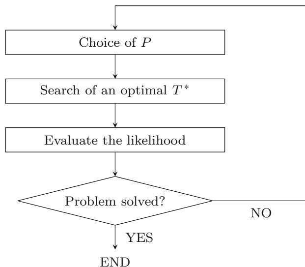
Fig. 3 Overview of our hybrid algorithm GADAG
