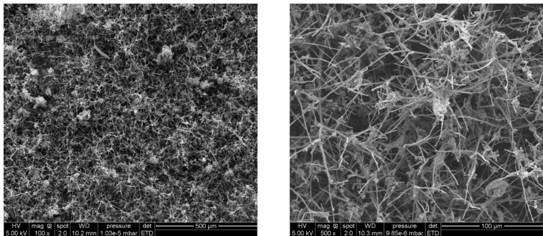
Fig. 4. SEM photographs (Jeol JSM-6380LV) of the microbial communities fouling plasterboard samples after 14 weeks. Left: magnification \times 100 ; Right: magnification \times 500 .
