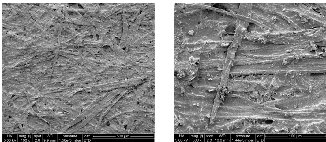
Fig. 5. SEM photographs (Jeol JSM-6380LV) of uncontaminated plasterboard samples after 14 weeks. Left: magnification \times 100 ; Right: magnification \times 500 .
