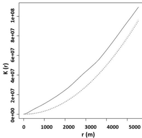
Figure 3. Ripley's K function for the observed HTOF. Dotted and dashed lines stand for 97.5% and 2.5% envelopes corresponding to complete spatial random point patterns
