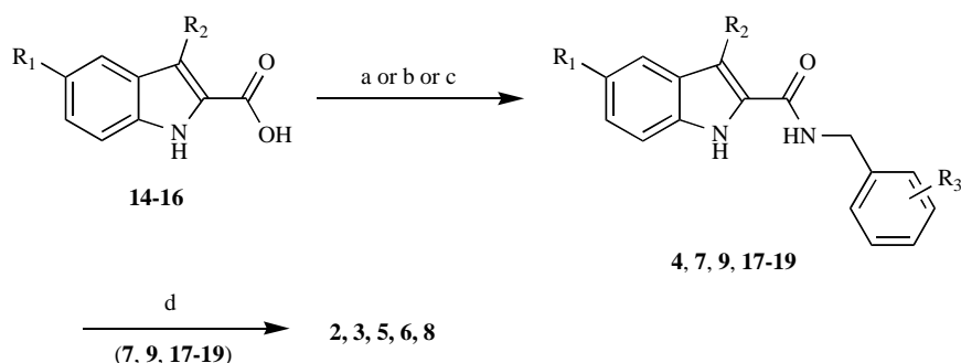
Scheme 2. Chemical synthesis of compounds 2-9 (Table 1); 14 : R 1 = Cl, R 2 = Ph; 15 : R 1 = Cl, R 2 = H; 16 : R 1 = Br, R 2 = H; 17 : R 1 = Cl, R 2 = H, R 3 = 3-NO 2 ; 18 : R 1 = Br, R 2 = H, R 3 = 3-NO 2 ; 19 : R 1 = Cl, R 2 = Ph, R 3 = 3-NO 2 . Reagents and conditions: (a) ( 4 , 10 , 11 ) amine, BOP reagent, TEA, anhydrous DMF, 25 °C, 12 h, 47-81%; (b) ( 9 , 12 ) (i) 1,1'-carbonyldiimidazole, anhydrous THF, 25 °C, 2 h; (ii) amine, 25 °C, 2 h, 42-59%; (c) ( 7 ) amine, PyBOP reagent, TEA, anhydrous DMF, 25 °C, 12 h, 30%; (d) SnCl 2 ·2H 2 O, AcOEt, 80 °C, 3 h, 54-87%.
