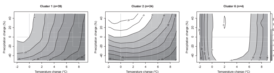
Figure 1. Ensemble mean changes in winter wheat grain yield (%) relative to the 1981-2010 baseline for the three dominant patterns of response identified using a hierarchical clustering approach across all study sites
