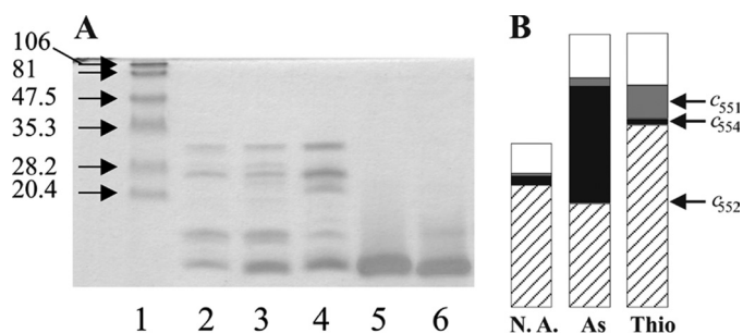
FIGURE 5. A, 3,3',5,5'-tetramethyl-benzidine-stained SDS-PAGE of cytochromes present in the S22 periplasm under different growing conditions. Lane 1, molecular weight standards; lane 2, cyts expressed without any addition; lane 3, cyts expressed in the presence of 5 mM \text{As}^{\text{III}} ; lane 4, cyts expressed in the presence of 20 mM thiosulfate; lane 5, purified cyt c_{554} ; lane 6, purified cyt c_{552} . B, schematic representation of cyt content of the DEAE-cyt fraction under different growing conditions. Lane N.A., cyt content without any addition; lane As, cyt content with 5 mM \text{As}^{\text{III}} ; lane Thio, cyt content with 20 mM thiosulfate. Note that the DEAE-cyt fraction represent only part of the total cyt fraction (see "Experimental Procedures") and that ~20% of cyt content in this DEAE-cyt fraction remains unidentified under each of the growth conditions.
