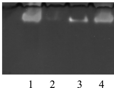
FIGURE 1. Polyacrylamide gel electrophoresis and in-gel Aro activity staining of subcellular fractions of S22. Lane 1, spheroplasts; lane 2, periplasm; lane 3, membrane fraction after French press treatment; lane 4, soluble fraction after French press treatment.
