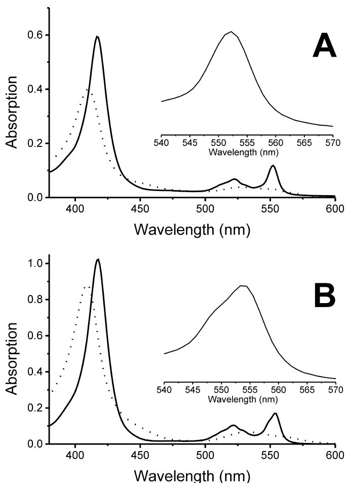
FIGURE 3. Spectra of c_{552} and c_{554} cytochromes enzymatically reduced by purified Aro. Oxidized cyts (black lines) were incubated for 3 min with the enzyme (dotted lines); c_{552} (A) and c_{554} (B). Insets show the \alpha -bands of cytochrome c_{552} and c_{554} absorbing at 552 and 554 nm, respectively.
