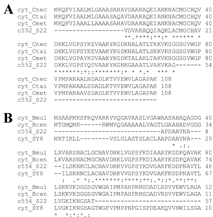
FIGURE 4. Sequence alignment of cytochromes purified from S22. The N-terminal sequence of purified cyt c_{552} ( c_{552\_S22} ; A) is compared with the sequences of cyts from Cupriavidus necator H16 (cyt_Cnec; GenBank™ accession no. YP_727996), C. taiwanensis (cyt_Ctai; GenBank™ accession no. YP_002007005) and C. metallidurans CH34 (cyt_Cmet; GenBank™ accession no. YP_585565), whereas the N-terminal sequence of c_{554} ( c_{554\_S22} ; B) is compared with the sequences of cyts from Achromobacter sp. SY8 (cyt_SY8; GenBank™ accession no. ABP63661), Burkholderia multivorans (cyt_Bmul; GenBank™ accession no. YP_001578392) and B. cenocepacia (cyt_Bcen; GenBank™ accession no. YP_002229329).
