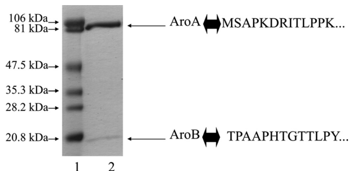
FIGURE 2. Coomassie Blue-stained SDS-PAGE on purified Aro from S22. Lane 1, molecular weight standards; lane 2, purified enzyme. Identification of subunits was confirmed by N-terminal sequencing.
