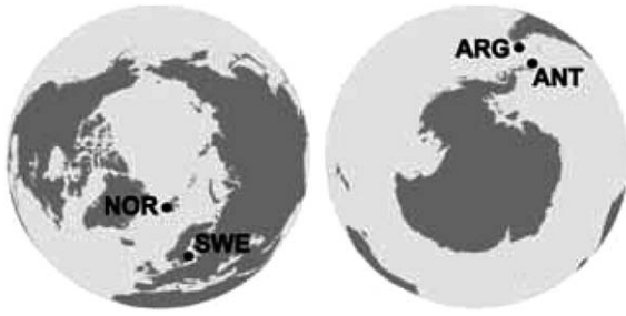
Fig. 1. Geographic location of the analysed sampling regions. NOR, Advent Fjord, Spitsbergen, Svalbard Archipelago, Norway; SWE, Port Värtahamnen, Stockholm, Baltic Sea, Sweden; ARG, Ushuaia Bay, Tierra del Fuego Island, Argentina; ANT, Potter Cove, 25 de Mayo (King George) Island, Antarctica. Two sampling sites distanced ~500 m were selected within each coastal environment, and the top 5 cm of subtidal sediments were sampled in triplicate within each site.
