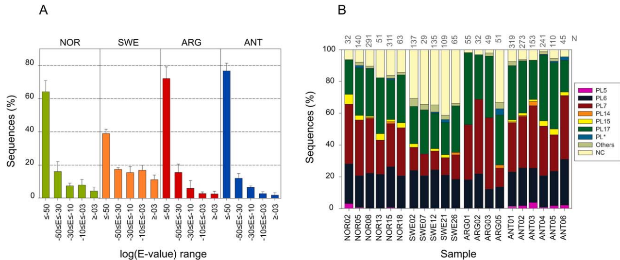
Fig. 4. Characteristics of the metagenomic ALH sequence dataset.
