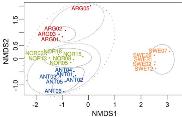
Fig. 3. Similarity of metagenomes based on shared ALH sequences.
