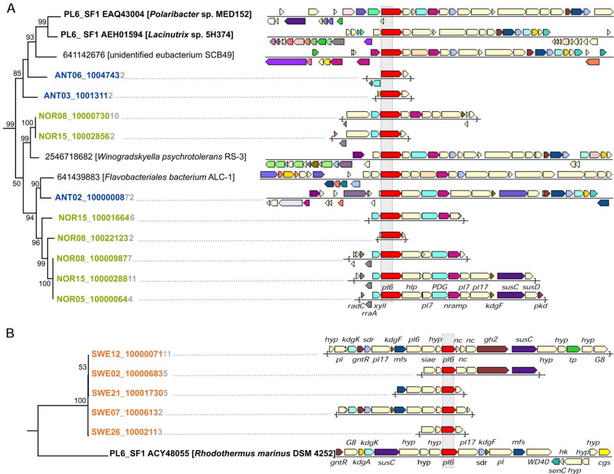
Fig. 5. Phylogenetic analysis of full-length ALH sequences and scaffold gene organization.
