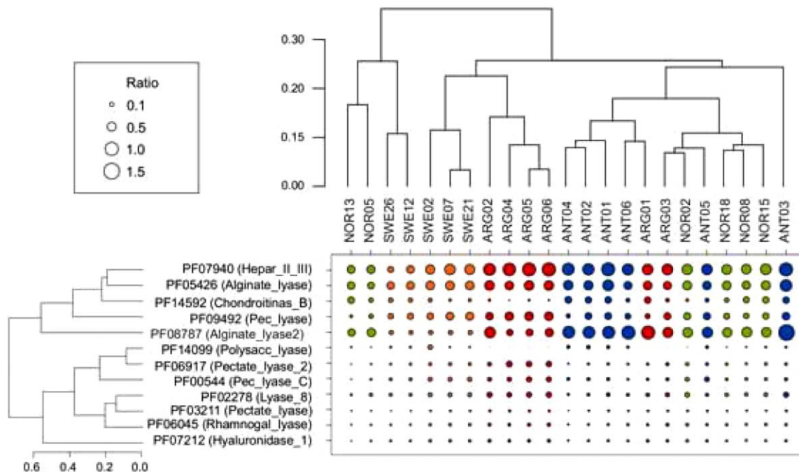
Fig. 2. Relative abundance of sequences containing Pfam domains from PL in the sediment metagenomes.
