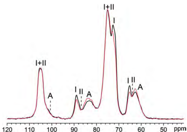
Fig. 3 Solid-state 13 C CP-MAS NMR spectra of α-cellulose untreated (black) and after regeneration on the D/S solvent system (red). I, II, and A indicate signals characteristics of cellulose type I, cellulose type II, and amorphous cellulose, respectively
