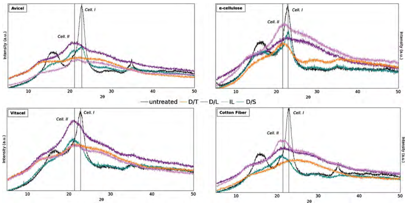
Fig. 2 XRD diffractograms showing different crystallinity forms between the different commercial and regenerated cellulose samples
