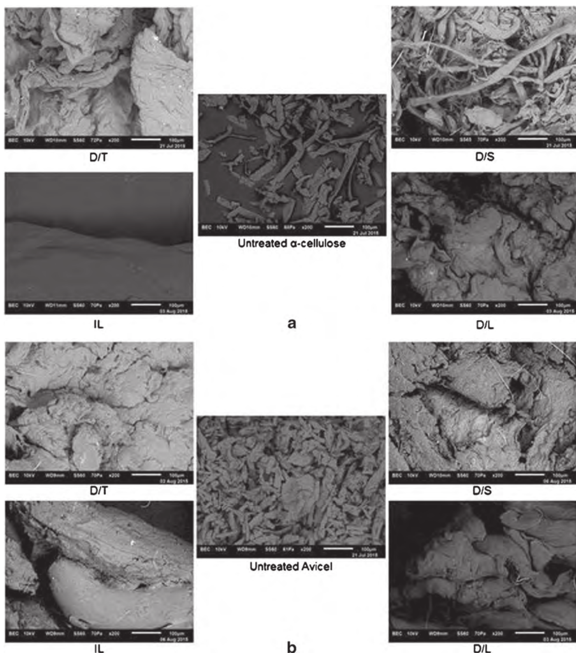
Fig. 1 SEM micrographs of \alpha -cellulose (a) and Avicel (b), untreated and regenerated after dissolution through the different solvent systems ( \times 200 with \rightarrow 100 \mu\text{m} )
