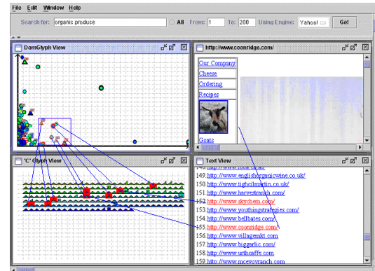
Figure 2 - An ad-hoc coordination example of Web Search Results Visualization [5]
