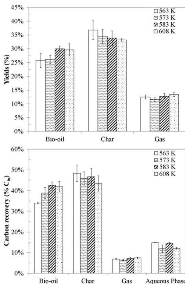
Fig. 2. Effect of reaction temperature on products distribution and carbon recovery (holding time = 60 min).
