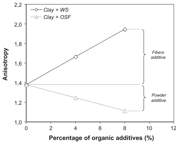
Fig. 5. Anisotropy of the clay ceramic and of the clay ceramic with a 4 wt% and an 8 wt% addition of OSF and WS after a firing process at 900 °C.
