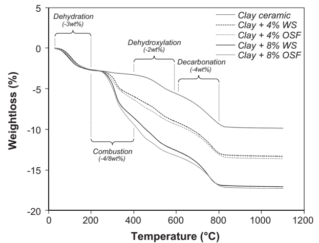
Fig. 2. Thermal behavior of the clay ceramic and of the clay ceramic with a 4 wt% and an 8 wt% addition of OSF and WS.
