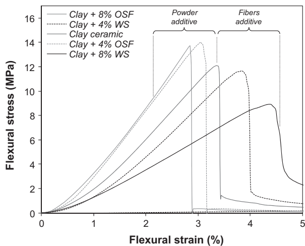
Fig. 7. Flexural stress-strain curves of the clay ceramic and of the clay ceramic with a 4 wt% and an 8 wt% addition of OSF and WS after a firing process at 900 °C.
