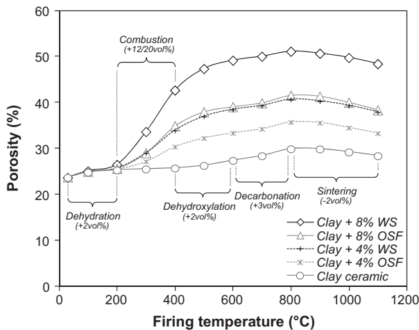
Fig. 3. Evolution of the porosity of the clay ceramic and of the clay ceramic with 4 wt% and an 8 wt% addition of OSF and WS with the firing temperature.
