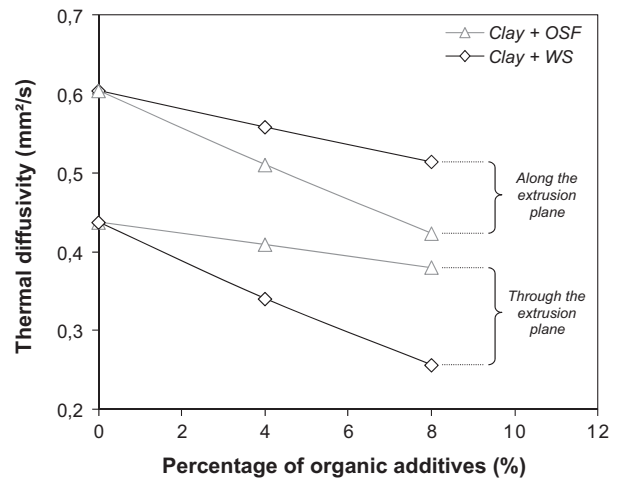
Fig. 6. Thermal diffusivity of the clay ceramic and of the clay ceramic with a 4 wt% and 8 wt% addition of OSF and WS after a firing process at 900 °C.
