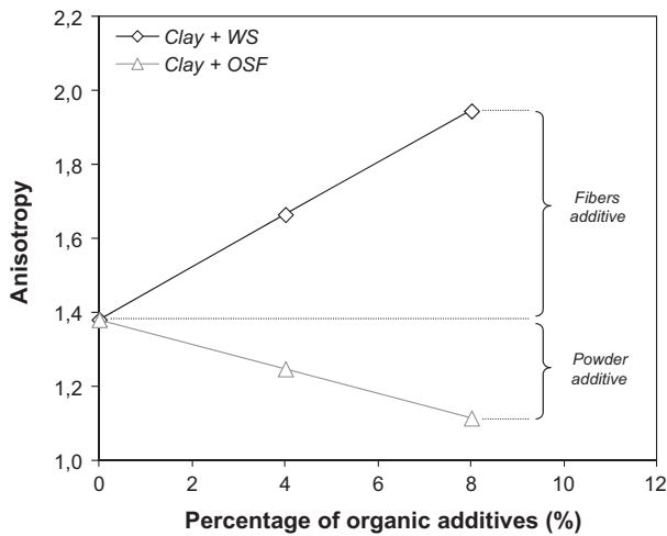
Fig. 5. Anisotropy of the clay ceramic and of the clay ceramic with a 4 wt% and 8 wt% addition of OSF and WS after a firing process at 900 °C.
