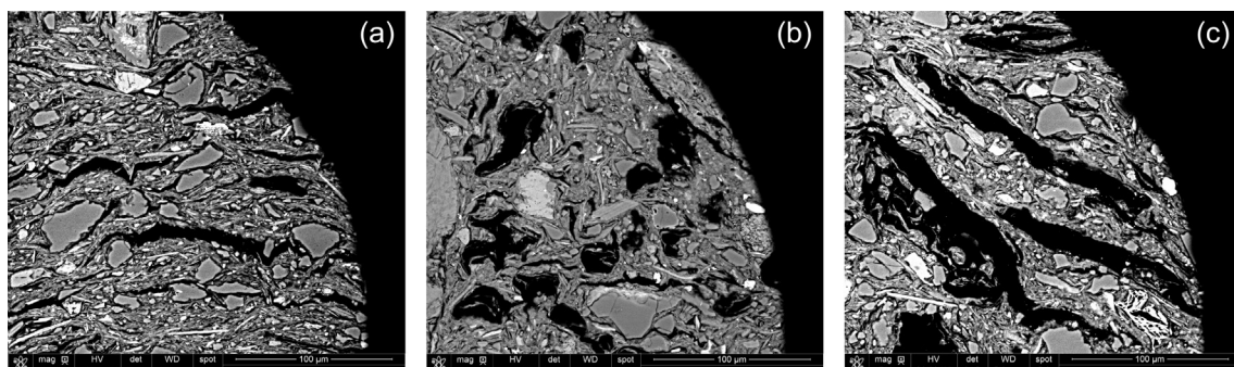
Fig. 4. SEM micrographs of the microstructure of the clay ceramic (a) and of the clay ceramic with an 8 wt% addition of OSF (b) and WS (c) after a firing process at 900 °C.
