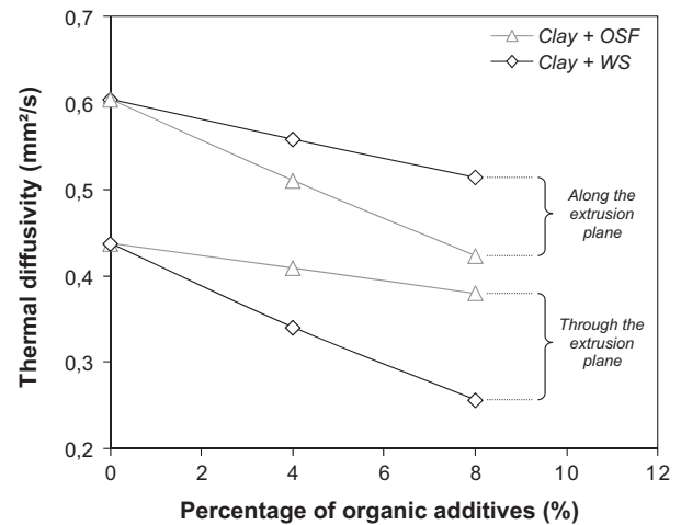
Fig. 6. Thermal diffusivity of the clay ceramic and of the clay ceramic with a 4 wt% and an 8 wt% addition of OSF and WS after a firing process at 900 °C.
