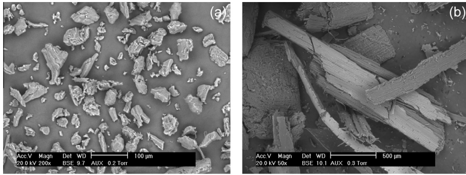
Fig. 1. SEM micrographs of the particle shape of OSF (a) and WS (b).
