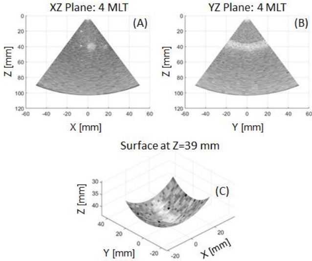
Figure 3: 3D results for 4 MLT.
