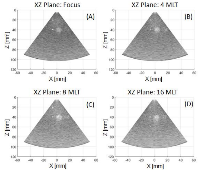
Figure 4: Comparison XZ planes for focus (A), 4 MLT (B), 8 MLT (C) and 16 MLT (D)
