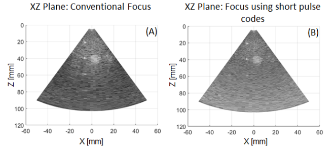
Figure 2: Focus sequence: XZ plane obtained by using 3 cycle signal (A), short coded pulse (B)
