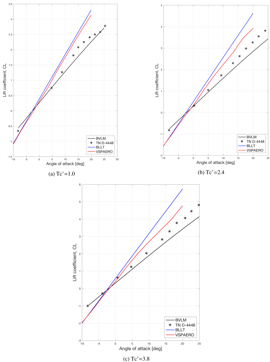
Figure 8: Comparison of the experimental and computational C_L - \alpha curves for three different thrust coefficients
