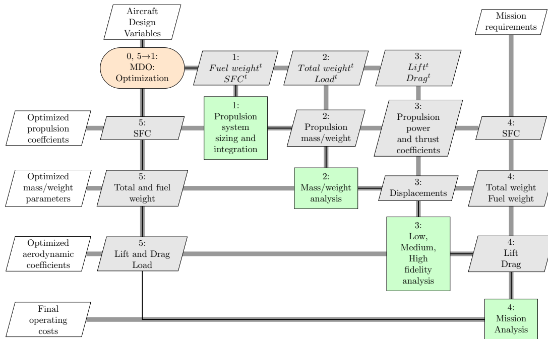
Figure 1: Multidisciplinary design optimization (MDO) workflow process
