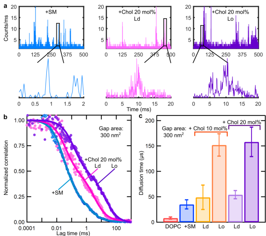
Figure 3. FCS measurements recorded in nanogaps of 300 \text{ nm}^2 area for binary and ternary lipid mixtures. (a) Fluorescence intensity time traces of DiD diffusion in DOPC:SM (1:1) (left, blue) and DOPC:SM (1:1) + Chol (20 mol%) in the Ld (middle, magenta) and Lo (right, purple) phases. Enlarged views of single bursts are also depicted for visual comparison. (b) Normalized ACF curves for the different lipid mixtures. (c) Mean diffusion times of the four probed lipid membranes \pm 1\text{std} obtained for the smallest gap area ( 300 \pm 48 \text{ nm}^2 ). Number of measurements: 20 for DOPC; 19 for DOPC:SM; 18 and 15 for Ld and Lo, respectively with Chol 10 mol%; and 17 and 15 for Ld and Lo, respectively with Chol 20 mol%. Between 5 and 10 different antennas of 300 \text{ nm}^2 area on 4 to 5 different samples were used for each lipid composition.
