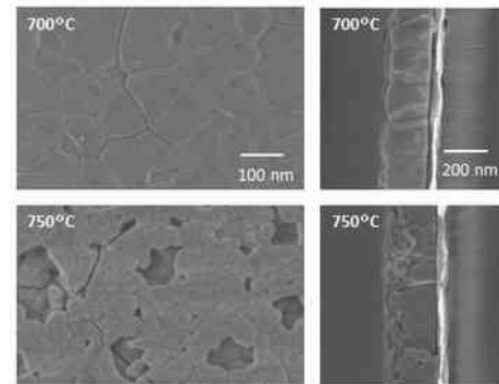
Figure 2: SEM micrographs of BNT thin films.
