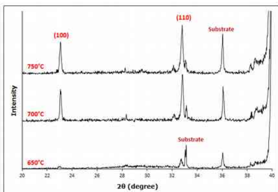
Figure 1: XRD patterns of BNT thin films.
