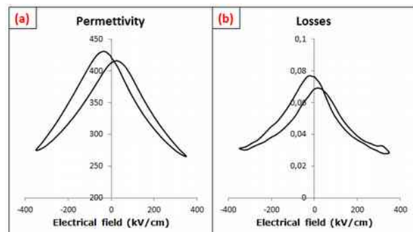
Figure 3: Electrical field dependences of (a) the permittivity and (b) the dielectric losses for the BNT thin film.
