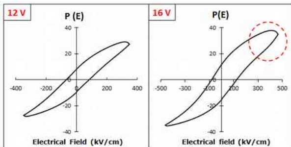
Figure 4: Room temperature macroscopic ferroelectric hysteresis (P-E) loops measured for a BNT film, for an applied voltage of 12 and 16V.
