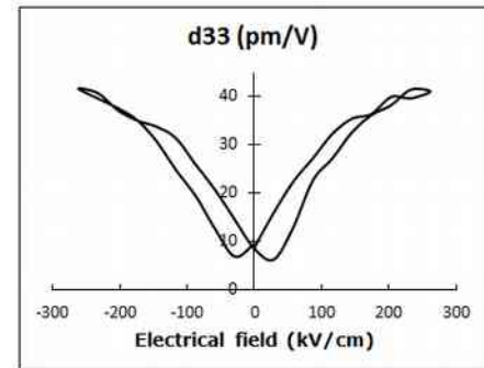
Figure 5: d_{33\text{eff}} (E) loop of BNT film.
