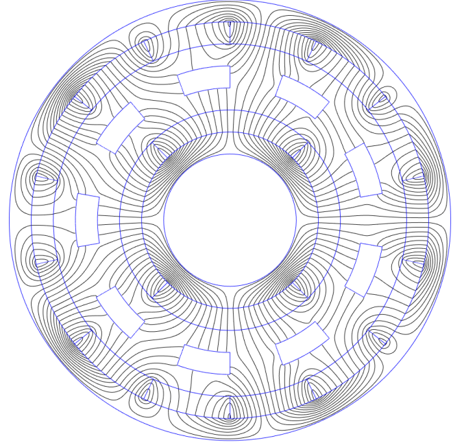
Fig. 4: 2-D representation of the magnetic flux line distribution in a magnetic gear obtained with the magnetostatic analytical model [18]. In this example: p_{int} = 2 , p_{ext} = 7 and Q = 9 (flux line distribution is not represented in pole pieces because the analytical model does not permit to compute the magnetic vector potential in these regions).
