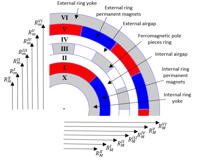
Fig.3. Magnetic gear parametrization of the different regions (in this example: p_{int} = 2 , p_{ext} = 7 and Q = 9 ).
