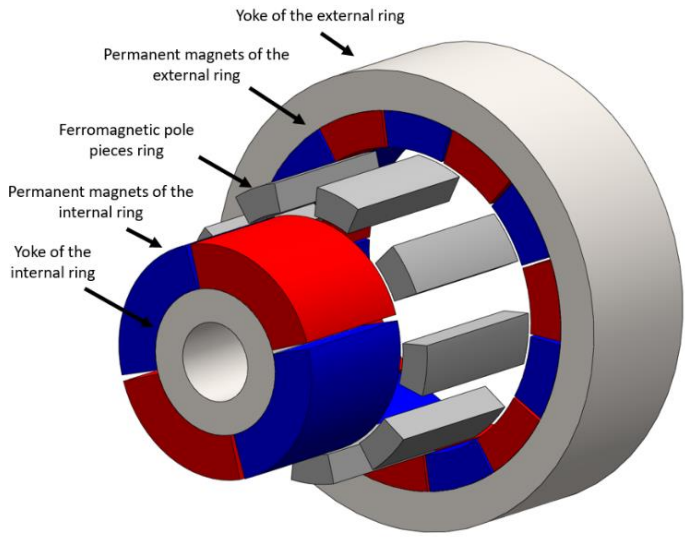
FigG.2. Magnetic gear architecture proposed by [6] in an exploded drawing with low pole numbers (in this example: p_{int} = 2 , p_{ext} = 7 and Q = 9 ).
