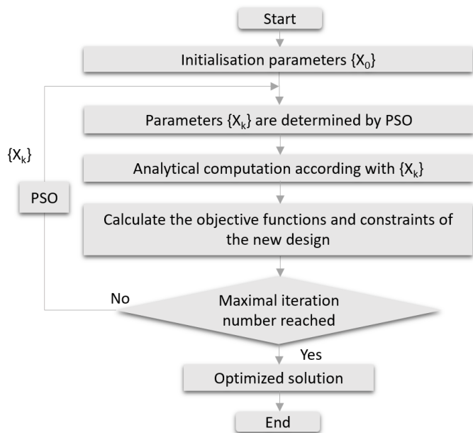
Fig. 6 Procedure of the optimization algorithm with the PSO (Particle Swarm Optimization) method.
