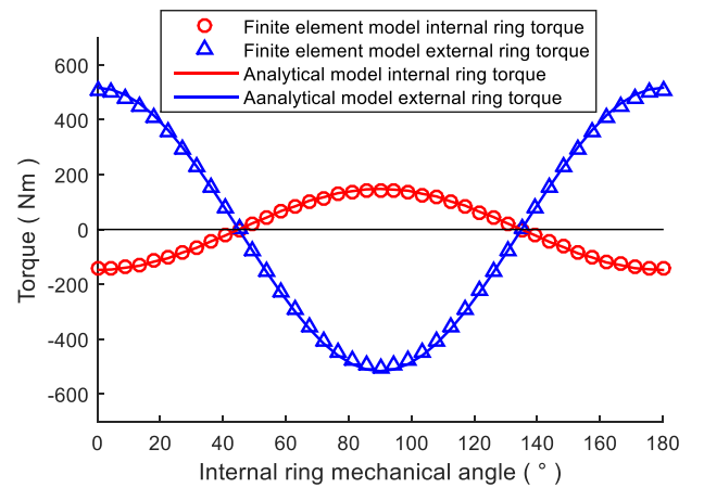
Fig.5: Magnetic torque evolution using an analytical model and a finite element model with a rotation of the internal ring while keeping the pole-piece ring and the external ring fixed for a magnetic gear with p_{int} = 2 , p_{ext} = 7 and Q = 9 .
