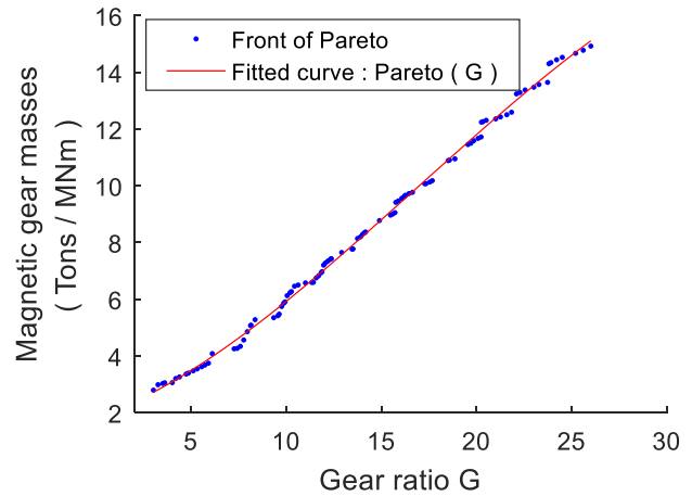
Fig. 7 Front of Pareto of the PSO bi-objective optimization with its order function three fitted curve for only one stage of magnetic gear and a constant external diameter.
