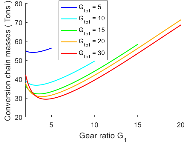
Fig. 8 Evolution of active mass of the FMID conversion chain with two magnetic gear stages versus the gear ratio ( G_1 ) of the first stage for the wind turbine presented in Table 4.
