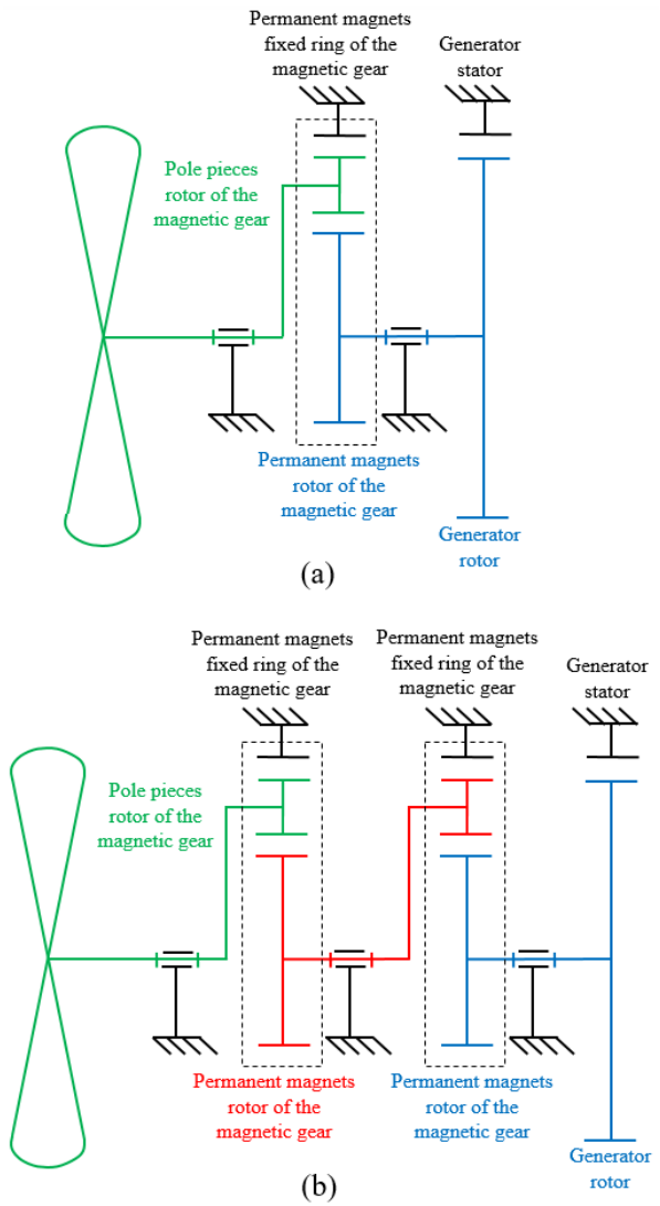
Fig. 1: Functional scheme of magnetic Indirect Drive (MID) conversion chain with (a) one stage of magnetic gear, (b) two magnetic gear stages.
