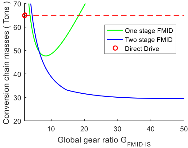
Fig. 9 Comparison between conversion chains composed of a single stage FMID, a two stages FMID and a direct drive with the same topology of hybrid excitation synchronous generator developed by Jeumont Electric for the wind turbine presented in Table 4.
