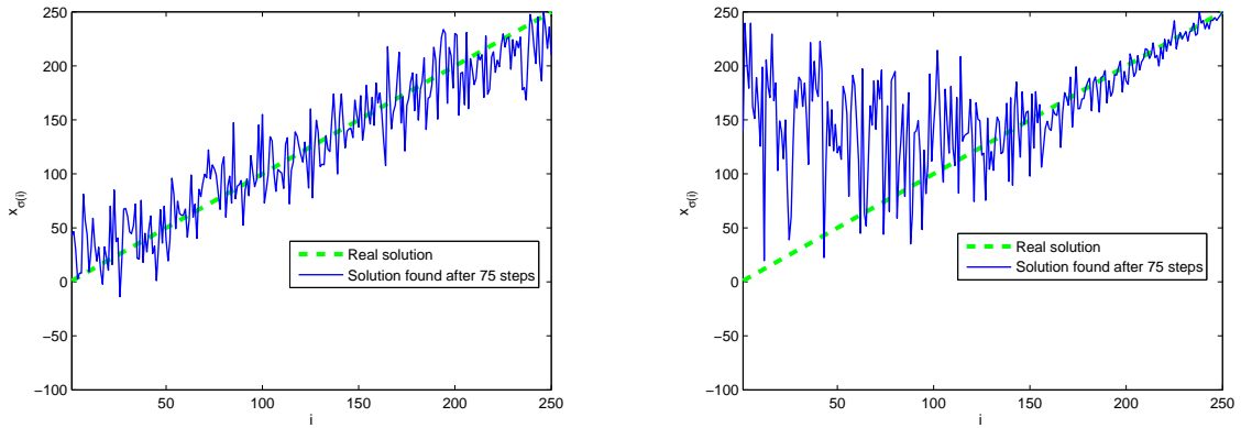
(a) Solution for test problem 1
