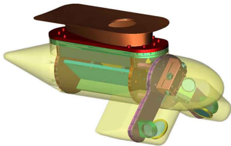
FIG. 2 (a) Front view of the Airborne interferometric Laser Imaging for Droplet Sizing probe (CL, SC: cylindrical, spherical lenses) and (b) 3D design of the probe [17]. The laser and the CCD sensor are in the main central part of the probe. The "two ears-extensions" include mirrors and windows. They allow to respect a scattering angle of \theta = 66^\circ , and a distance between the instrument and the measurement volume larger than 10 cm.
