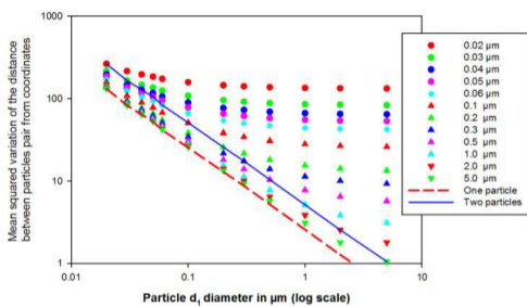
Figure 4.5: MSDV versus particle diameter.
