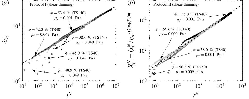
FIGURE 8. The evolution of the front position x_f^N for protocol I (a) and the variable X_f^N = (x_f^N/\eta_n)^{(2m+3)/m} for protocol II (b) as a function of time t^N in dimensionless form (5.3). The dashed lines (---) represent the self-similar solution (5.4) with m = 0.8 (i.e. x_f^{(s)N} \sim 1.39(t^N)^{0.17} ) (a) and X_f^N = t^N (b).
