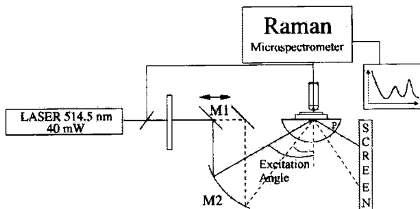
FIG. 4. Optical device used in micro-Raman experiment.
