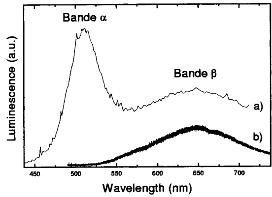
FIG. 9. Luminescence spectra of CdSe nanocrystals embedded in a bulk SiO 2 matrix (a) and of sample B (b).
