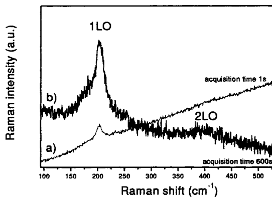
FIG. 8. Raman spectra obtained at 514.5 nm of CdSe nanocrystals embedded in a bulk SiO 2 matrix (a) and of sample A (b).
