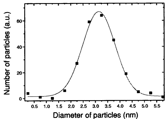
FIG. 2. Size distribution of CdSe nanocrystals embedded in the sol-gel SiO 2 ultrathin film (sample A).
