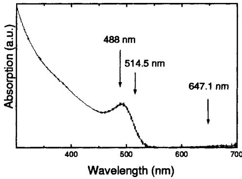
FIG. 7. Absorption spectra of CdSe nanocrystals embedded in a bulk SiO 2 matrix.
