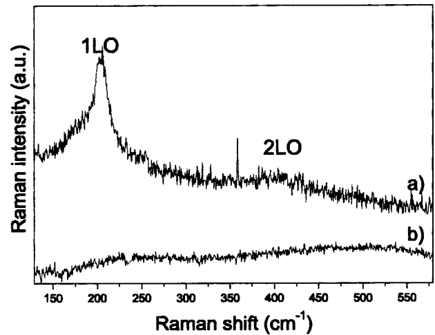
FIG. 5. Raman spectra of sample A in SPE configuration (a) and in conventional configuration (b).
