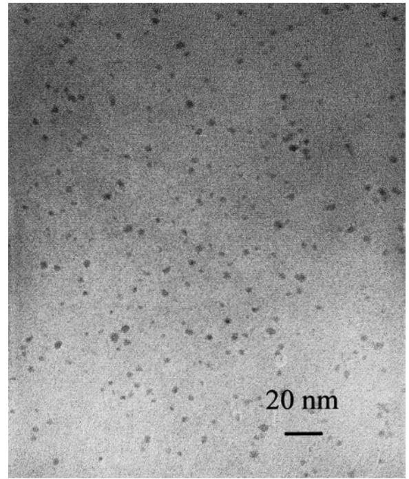
FIG. 1. CTEM micrograph of sample A.
