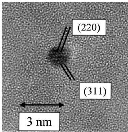
FIG. 3. Typical CdSe nanocrystals measured at 3 nm diameter embedded in the sol-gel matrix.
