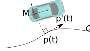
Figure 5: Map-matching of point M with spline \mathcal{C} defined by the vector of polynomial p(t) .
