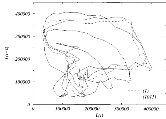
FIG. 20. The small sampling rate and the presence of many erratic oscillations prevent a correct counting of oriented crossings.
