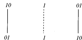
FIG. 21. The layering number N_{\text{lay}}(10,1) is found to be equal to +1.
