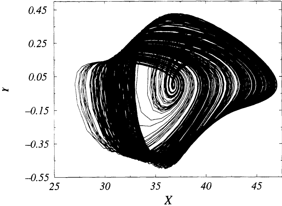
FIGURE 12. Reconstructed attractor of the iron electrodisso- lution obtained by integrating the reconstructed vector field.
