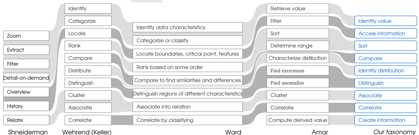
Fig. 16. Summary of the different task taxonomies that lead us to our proposal
