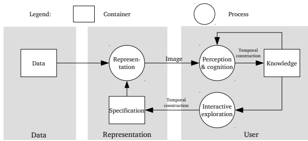
Fig. 1. The visualization process according to van Wijk
