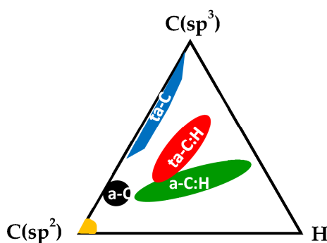
Figure 21. Basic ternary phase diagram of amorphous carbons.
