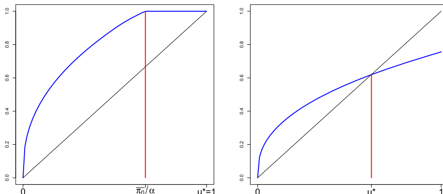
FIG 13. Plot of u \mapsto G_{W^*}^\infty(u) when \alpha \geq \bar{\pi}_0 (left panel) and \alpha < \bar{\pi}_0 (right panel).
