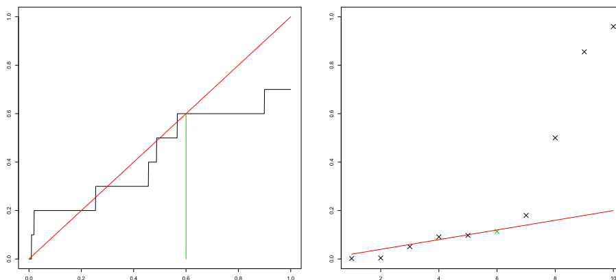
FIG 1. The BH procedure applied to a set of 10 p-values. Right plot: the p-values and the function k \rightarrow \alpha k/m . Left plot: identity function and \hat{G} . Each plot shows that 6 p-values are rejected.
