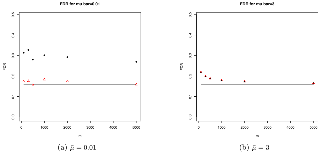
Fig 3: FDR against m in scenario 3. Group 1, ADDOW (black dots) and sADDOW _{\beta} (red triangles). Horizontal lines: \alpha and \pi_0\alpha levels.
