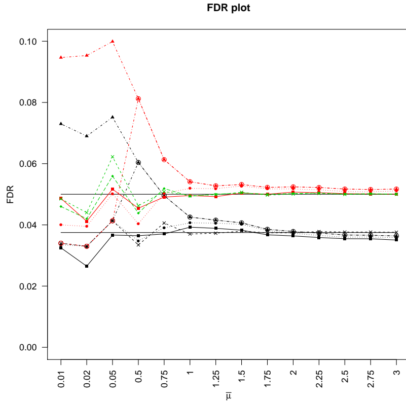
Fig 2: FDR against \bar{\mu} in scenario 1. Group 1 in black; Group 2 in green; Group 3 in red. The type of procedure is MWBH ( W_{\sigma_T}^* ) (squares); ADDOW (triangles); sADDOW _{\beta} (circles); Pro2 (disks); HZZ (diamonds) and finally BH/ABH (crosses). Horizontal lines: \alpha and \pi_0\alpha levels. See Section 6.1.
