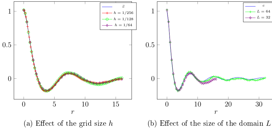
Figure 4: Comparison between isotropic covariance approximations, the periodic target covariance \tilde{c} , and the non-periodic version of \tilde{c} .
