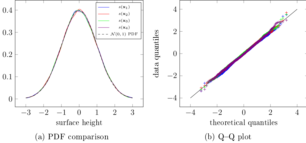
Figure 3: Verification of surface height distribution in four points on the surface
