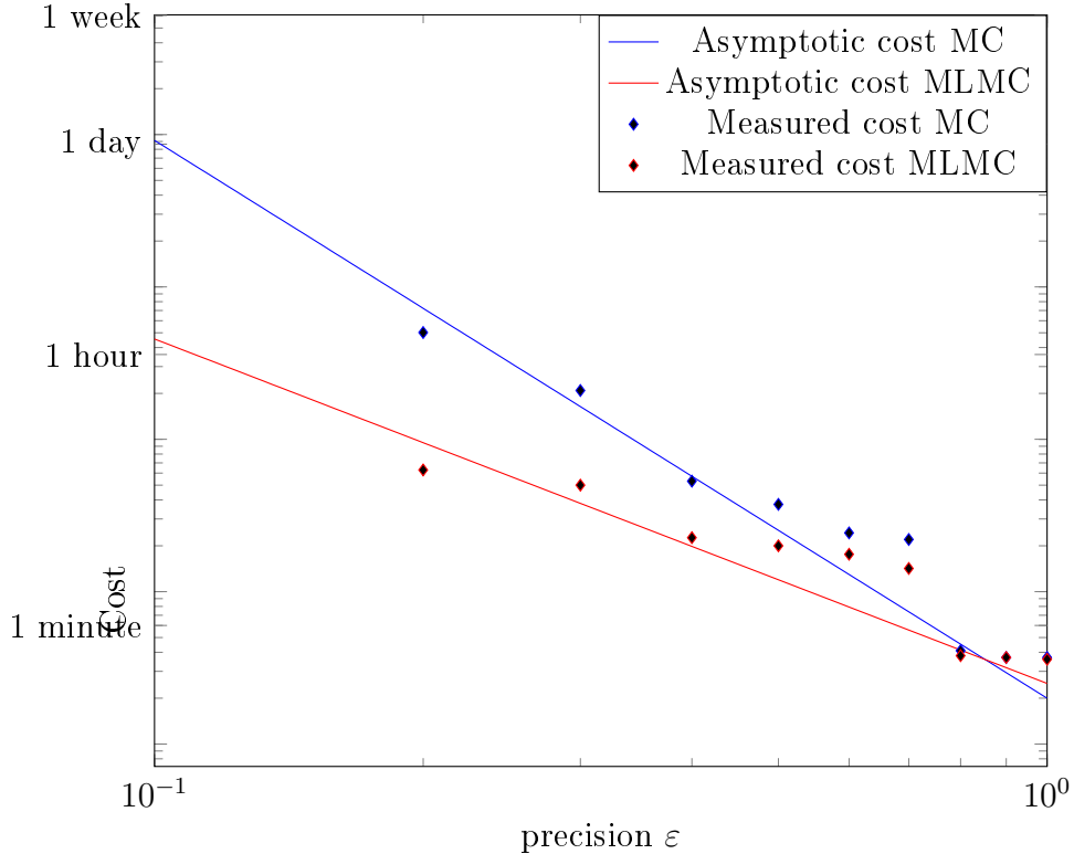
Figure 7: Theoretical and measured costs for the MC and the MLMC estimators for different tolerances. The quantity of interest is the contact area.
