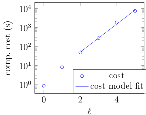
Figure 6: Estimation of the cost model.
