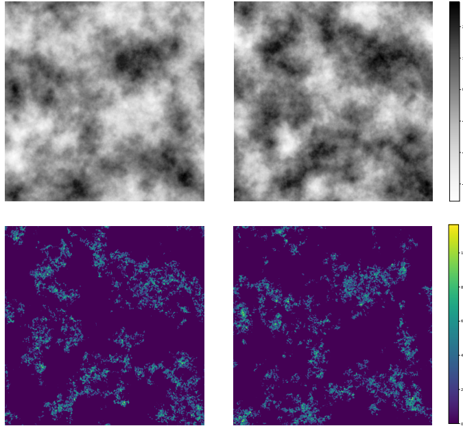
Figure 2: Typical pressure distributions (in color) obtained under a load \bar{p} = 10 corresponding to two different realizations of a rough random surface (in grey) defined by the same power spectrum.
