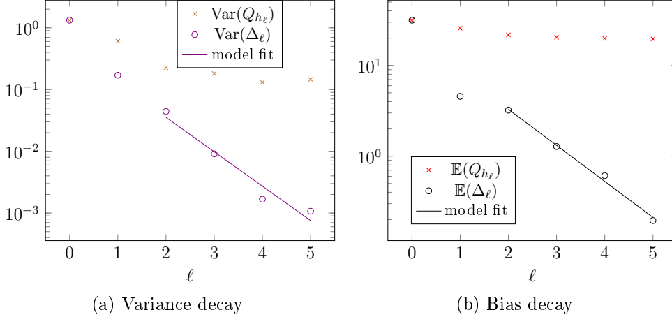
Figure 5: Estimation of convergence rates.
