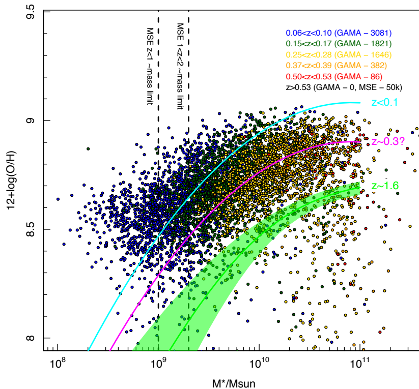
Figure 68: The mass-metallicity relation seen by GAMA and with the redshift ranges discussed in SRO-09 shown ( 0.12_{\text{sol}} lies at the lower limit of the plot). MSE will probe mass limits similar to GAMA at z < 0.1 and z < 0.2 but out to z < 1 and z < 2 respectively. The z < 0.1 mass – metallicity relation from SDSS+GAMA (Lara-Lopez, et al. 2013a) is displayed as the cyan line, the magenta line show the same relation normalized to the 0.25 < z < 0.39 sample and the green polygon shows the stacked galaxy z \sim 1.6 relation from Zahid et al. (2013). These observations clearly predict
