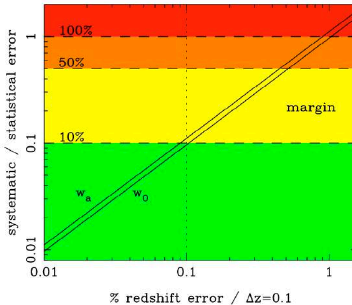
Figure 81: The predicted systematic error divided by the marginalised statistical error for parameters w_0 and w_a from Euclid BAO measurements (including the Planck data), required to normalise the BAO scale (solid lines). These are calculated for different values of the systematic error placed on the mean redshift in a bin of width \Delta z=0.1 . The requirement for Euclid is 0.1% (shows by the vertical dotted line) and can be verified with Euclid slitless spectroscopy using a sample of 140 000 galaxies with purity >99%. Ground based observations of a significant fraction of these same galaxies from a highly complete spectroscopic survey will play an important role. ( Figure from Laureijs et al. 2009 ).
