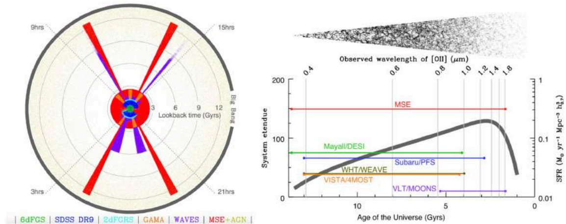
Figure 3: Left panel: Cone plot showing an example MSE survey compared to other notable benchmark galaxy surveys. Cones are truncated at the redshift at which L^* galaxies are no longer visible. Right panels: Lookback time versus cosmic star formation rate (right axis) using the parameterization of Hopkins & Beacom (2006). Grey lines indicate the wavelength of OII 3727\text{\AA} . Also indicated on this wavelength scale is the wavelength range of all highly multiplexed spectroscopic facilities in development. These are offset vertically according to their system etendue (left axis). The light cone demonstrates the reach of MSE for extragalactic surveys using a homogeneous set of tracers at all redshifts. See Chapter 3 for more details.
