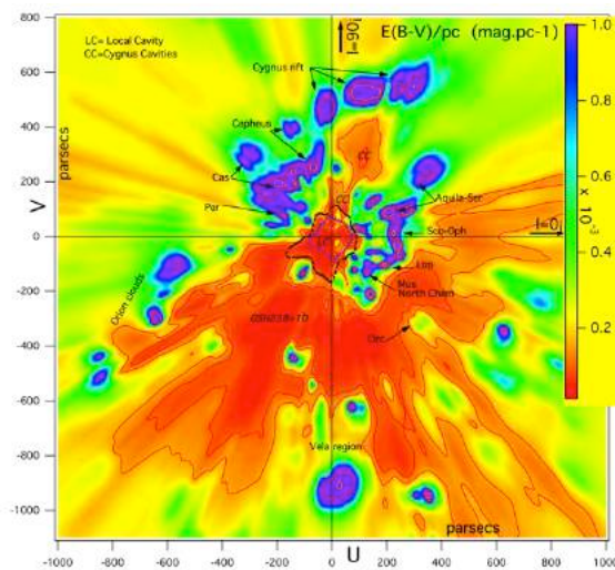
Figure 70: 3D mapping based on reddening measurements. Planar cut in the 3D opacity distribution inverted from 23 000 (wide + narrow)-band reddening measurements. The Sun is at (0,0). Units are parsecs, red is very low density and violet indicates dense areas. External areas with a homogenous color correspond to the absence of constraining (distance- and longitude-distributed) target stars. The local cavity at the center is surrounded by well-known cloud complexes and other cavities, including a huge region devoid of dust in the third quadrant. The
