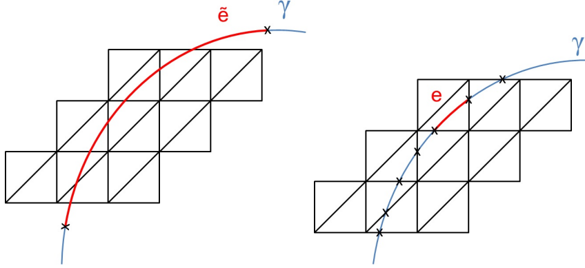
FIGURE 2. Example of meshes on \gamma .
