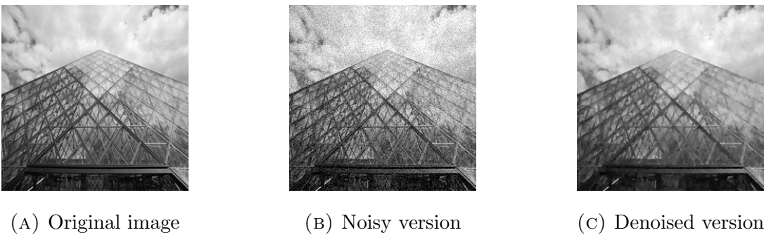
FIGURE 1. Original, noisy and TV-Huber denoised images used. Noise is Gaussian distributed with zero mean and variance \sigma^2 = 0.005 . The regularisation parameter is \lambda = 0.1 and the Huber parameter is \varepsilon = 0.01 so that \mu = 0.1 .
