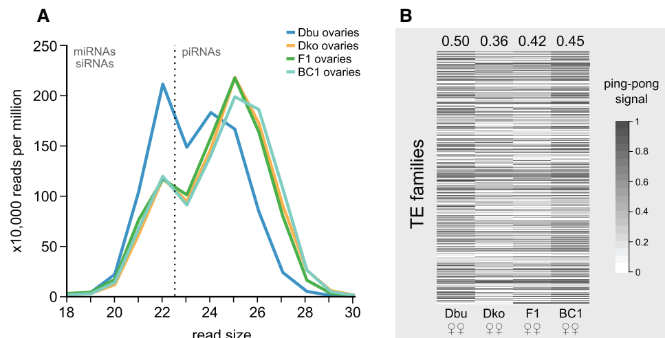
Fig. 5. —Characterization of piRNA populations in parental and hybrid ovaries. Dbu, D. buzzatii ; Dko, D. koepferae ; ♀♀, ovaries. (A) Read length distribution of ovarian small RNAs. The vertical dot line separates miRNAs and siRNAs (left) from piRNAs (right). (B) piRNA ping-pong fraction for each TE family (gray lines) and for the whole piRNA population (upper number). Only families with detectable ping-pong signal (>0) for at least one ovarian sample are represented.
